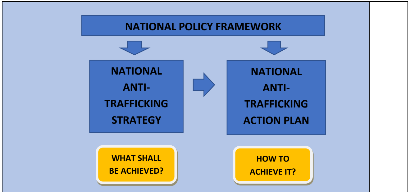
Fig. 1 - NPF Structure
